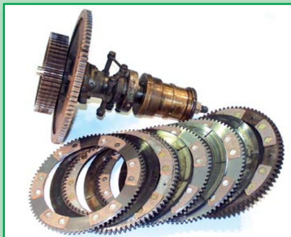
Clutch Bugatti 46 2T 1929 RENSPOINT 12060 - before assembling
